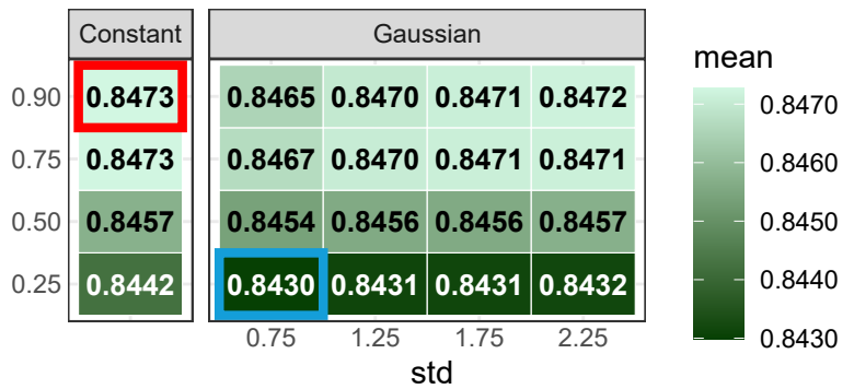
Jaccard
