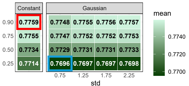
Sensitivity
