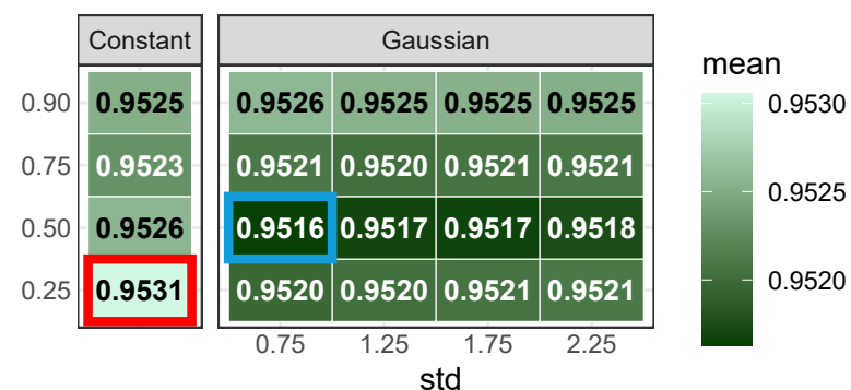
Specificity
